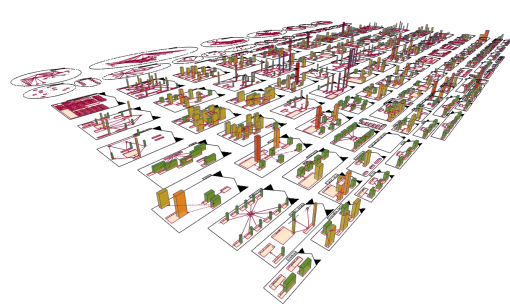
(b) UML City: UML diagram enriched with metrics
