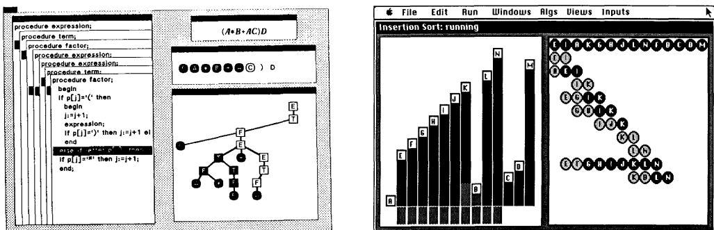
Figure 2.3. The Balsa (left) and Balsa-II (right) algorithm visualization systems
