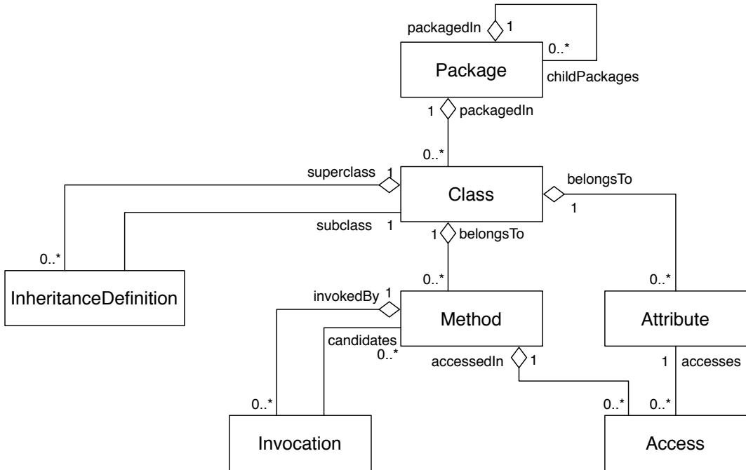
Figure 3.1. The core of the FAMIX meta-model
