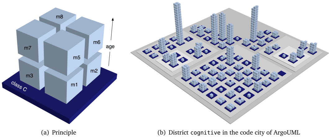
Figure 3.10. Fine-grained representation
