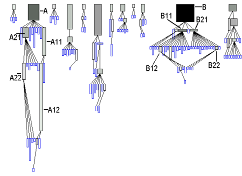
(b) Polymetric views in CodeCrawler
