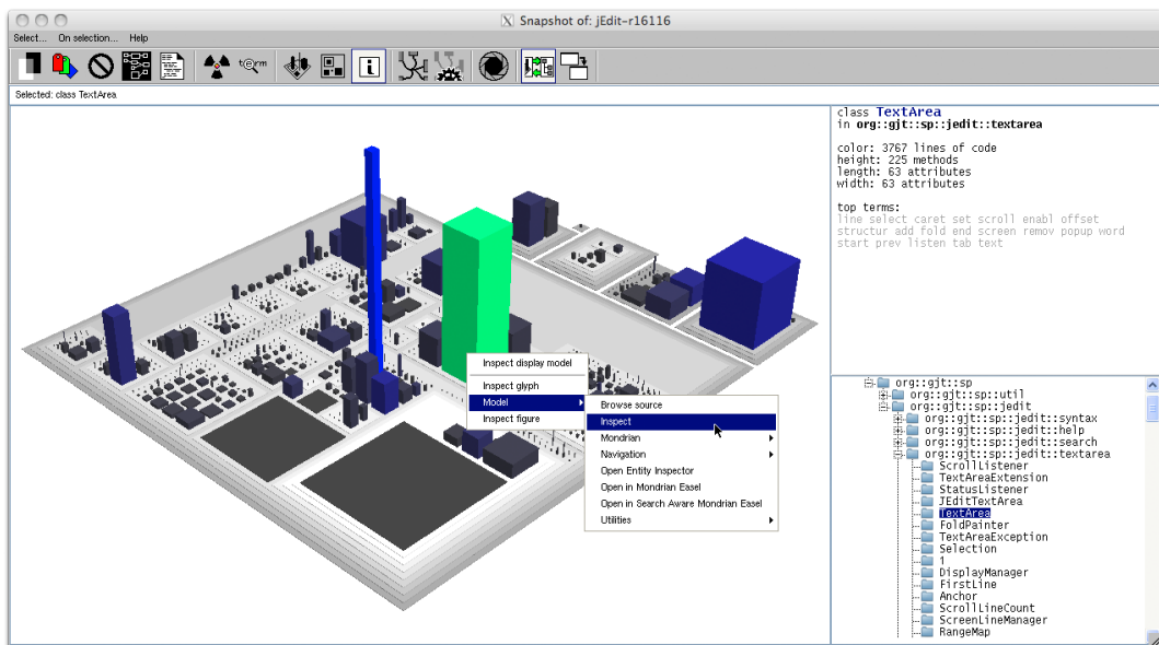
Figure 6.1. CodeCity's main window
