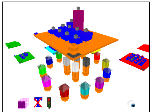
(b) Software visualized in a VR environment
