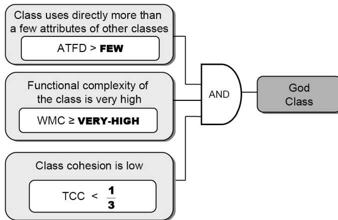
Figure 5.1. The God Class detection strategy [LM06]
